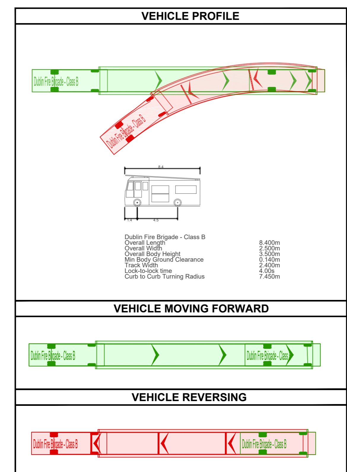
FIRE TENDER DUNDRUM ROAD JUNCTION NORTH (EXISTING) VEHICLE TRACKING SCALE @ A2: 1:400 SCALE @ A2: 1:800
