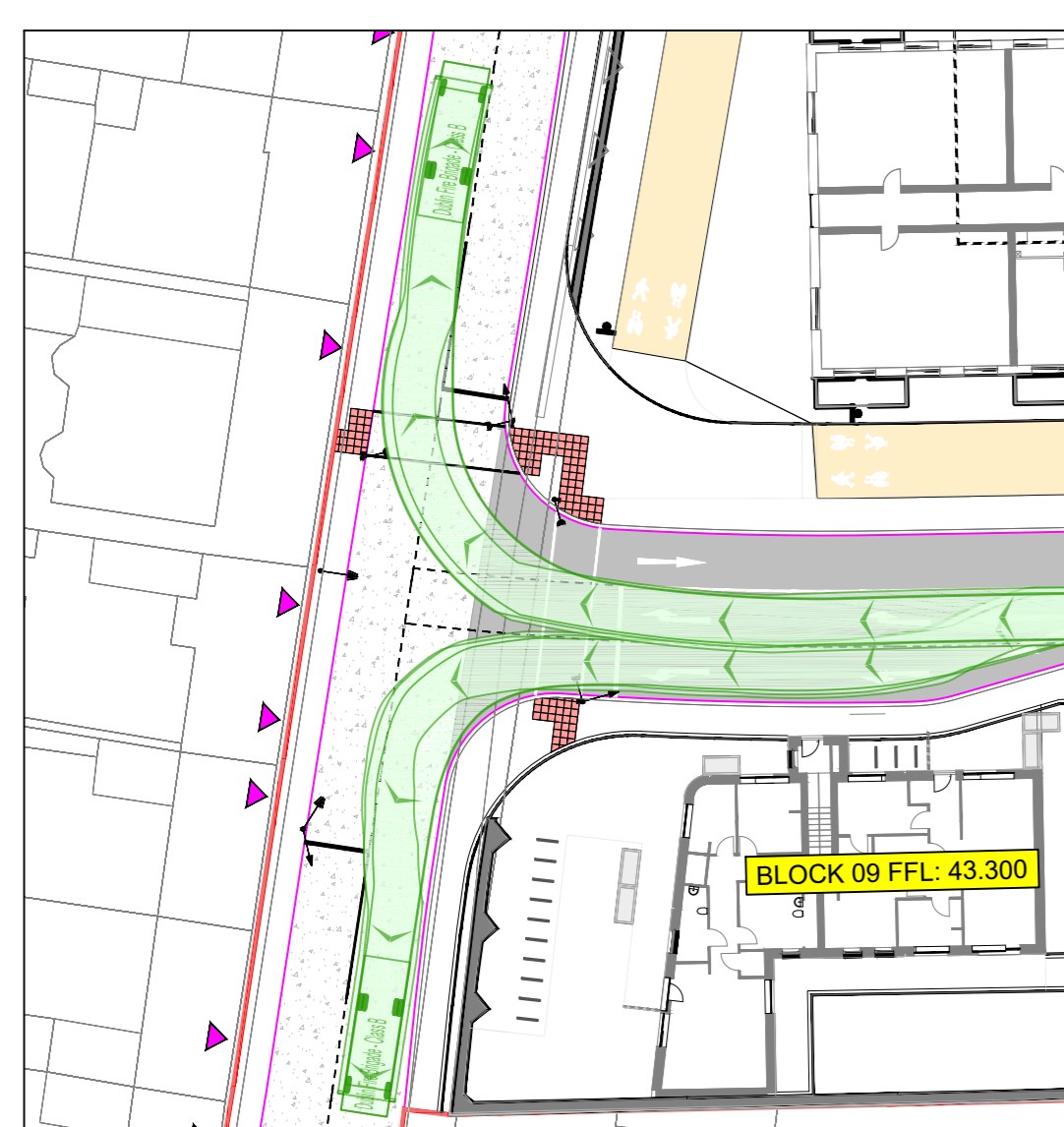
FIRE TENDER DUNDRUM ROAD JUNCTION SOUTH (EXISTING) VEHICLE TRACKING SCALE @ A2: 1:400 SCALE @ A2: 1:800
