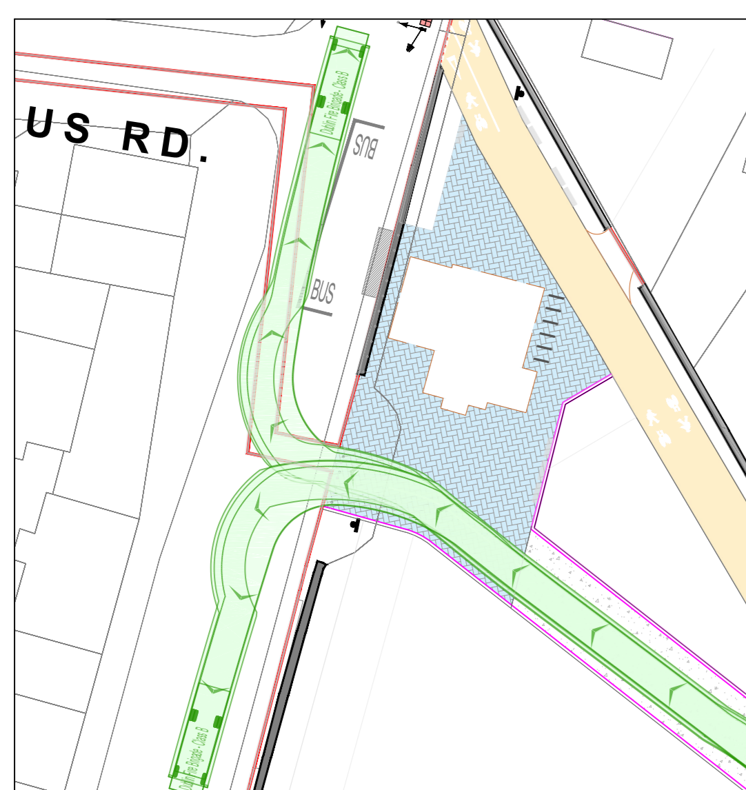
FIRE TENDER DUNDRUM ROAD JUNCTION NORTH (EXISTING) VEHICLE TRACKING SCALE @ A2: 1:400 SCALE @ A2: 1:800
